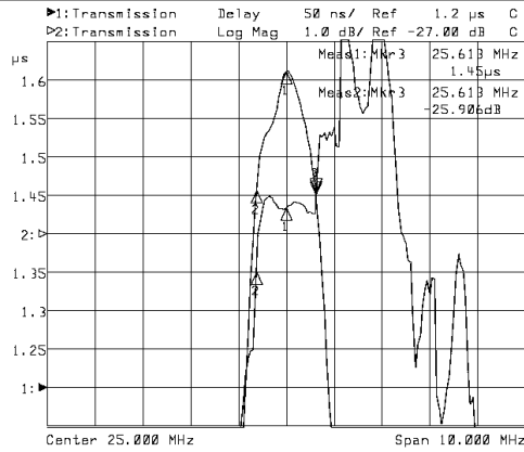
Horizontal: 1MHz/Div Vertical: 50nsec/Div&10dB/Div
