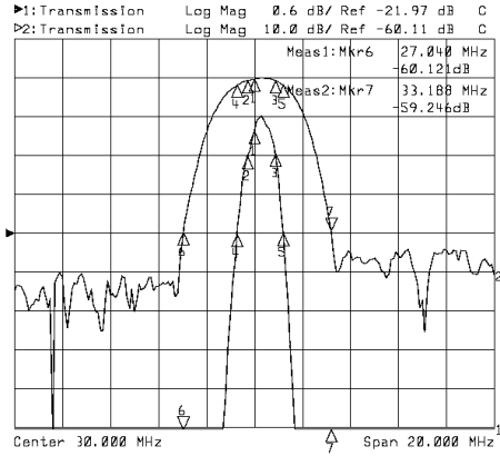
Horizontal: 2MHz/Div Vertical: 0.6dB/Div&10dB/Div
