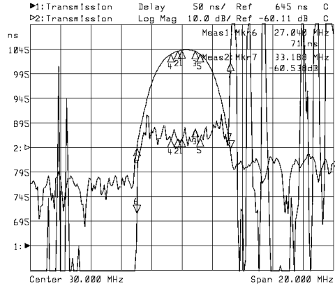
Horizontal: 2MHz/Div Vertical: 50ns/Div&10dB/Div
