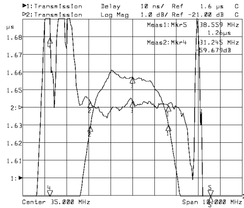
Horizontal: 1MHz/Div Vertical: 10nsec/Div&10dB/Div
