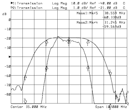
Horizontal: 1MHz/Div Vertical: 1dB/Div&10dB/Div
