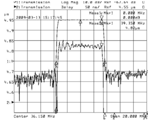
Horizontal: 2MHz/Div Vertical: 50nsec/Div&10dB/Div
