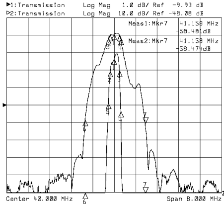
Horizontal: 0.8MHz/Div Vertical: 1dB/Div&10dB/Div
