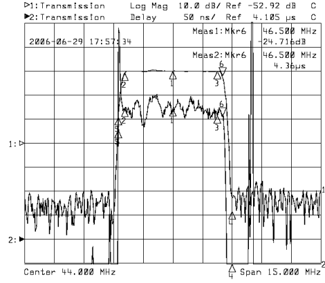
Horizontal: 1.5MHz/Div Vertical: 50nsec/Div&10dB/Div
