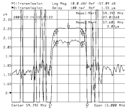
Horizontal: 1.5MHz/Div Vertical: 100ns/Div&10dB/Div
