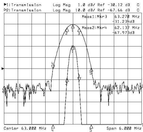
Horizontal: 0.6MHz/Div Vertical: 1dB/Div&10dB/Div
