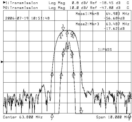
Horizontal: 1.0MHz/Div
