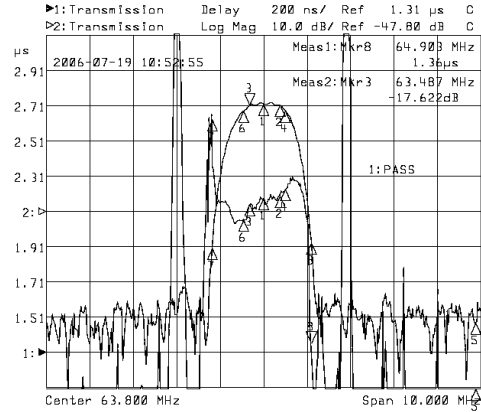
Horizontal: 1.0MHz/Div
