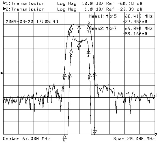
Horizontal: 2.0MHz/Div Vertical: 1dB/Div&10dB/Div
