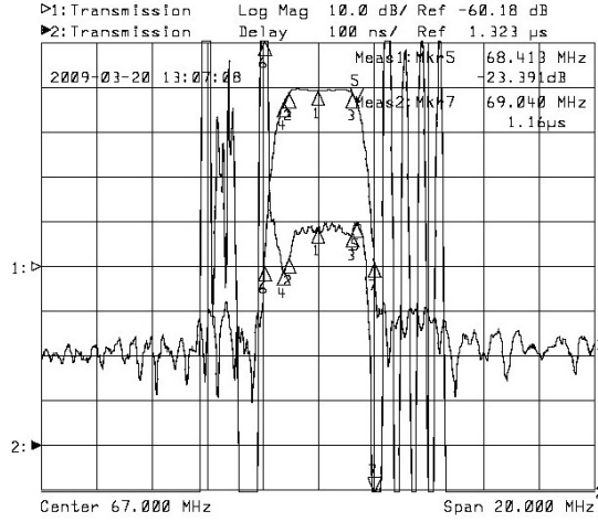
Horizontal: 2.0MHz/Div Vertical: 100nS/Div&10dB/Div
