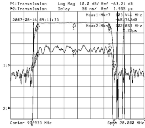
Horizontal: 2MHz/Div Vertical: 50ns/Div&10dB/Div
