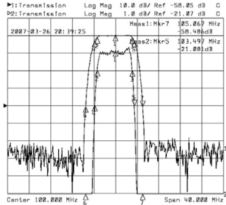
Horizontal: 4MHz/Div Vertical: 1dB/Div&10dB/Div
