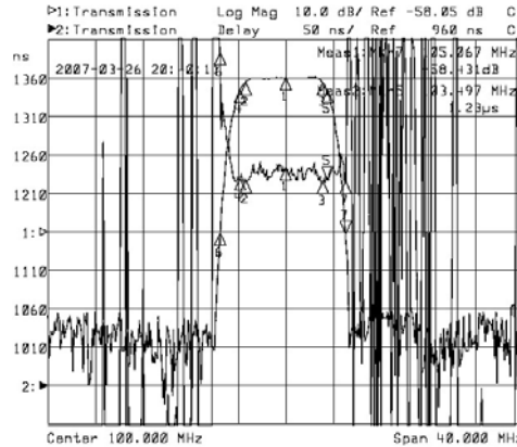
Horizontal: 4MHz/Div Vertical: 50nsec/Div&10dB/Div
