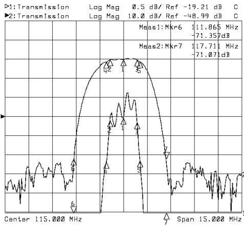
Horizontal: 1.5MHz/Div Vertical: 1dB/Div&10dB/Div
