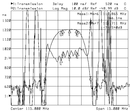
Horizontal: 1.5MHz/Div Vertical: 100ns/Div&10dB/Div
