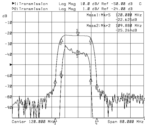
Horizontal: 8MHz/Div Vertical: 1dB/Div&10dB/Div
