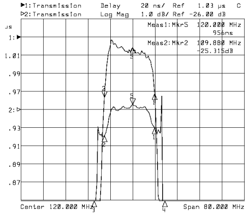
Horizontal: 8MHz/Div Vertical: 20nsec/Div&10dB/Div
