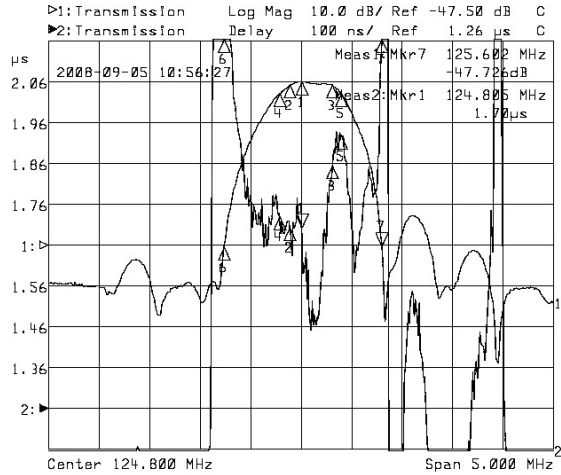
Horizontal: 0.5MHz/Div Vertical: 100nsec/Div&10dB/Div
