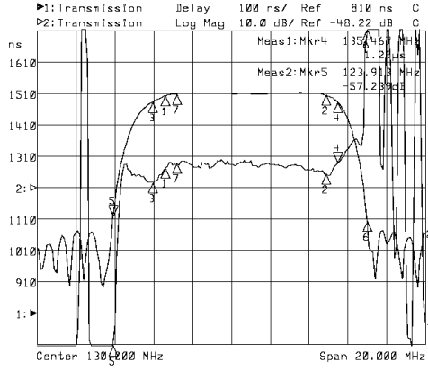
Horizontal: 2MHz/Div Vertical: 100nsec/Div&10dB/Div
