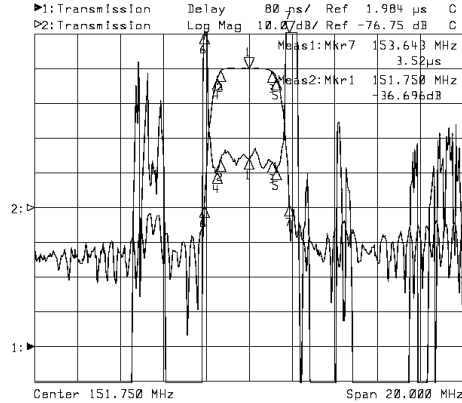
Horizontal: 2MHz/Div Vertical: 80nsec/Div & 10dB/Div
