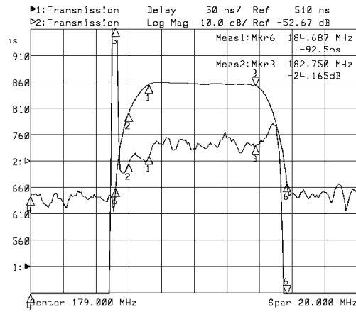
Horizontal: 2.0MHz/Div Vertical: 50nsec/Div & 10dB/Div
