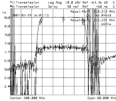
Horizontal: 8MHz/Div Vertical: 50nsec/Div&10dB/Div
