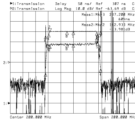
Horizontal: 20MHz/Div Vertical: 50ns/Div & 10dB/Div
