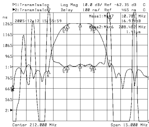
Horizontal: 1.5MHz/Div Vertical: 100ns/Div & 10dB/Div
