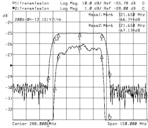
Horizontal: 15MHz/Div Vertical: 10dB/Div & 1dB/Div
