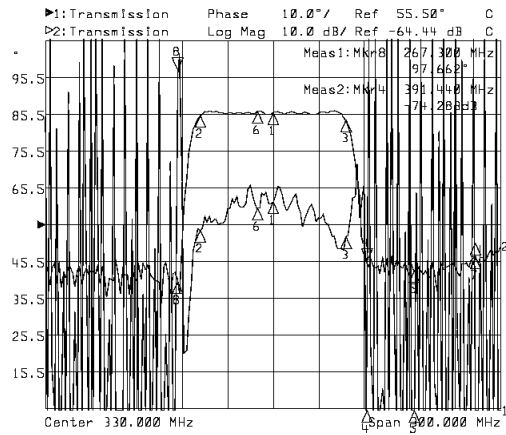
Horizontal: 30MHz/Div Vertical: 10°/Div
