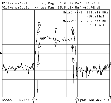
Horizontal: 30MHz/Div Vertical: 10dB/Div
