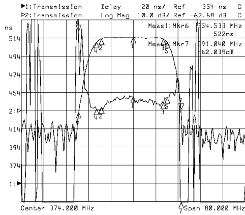
Horizontal: 80MHz/Div Vertical: 20ns/Div & 10dB/Div
