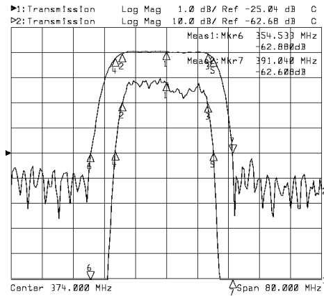
Horizontal: 80MHz/Div Vertical: 10dB/Div&1dB/Div
